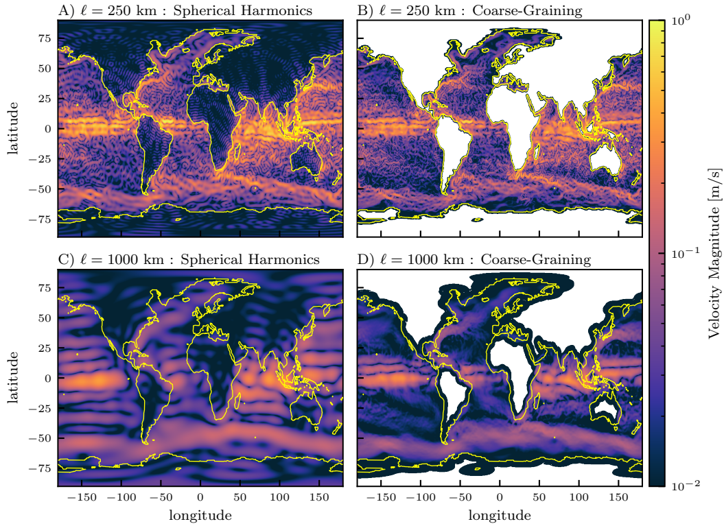
Figure 4. Filtering Maps with Spherical Harmonics and Coarse-Graining Speed of the large-scale AVISO surface currents obtained by [left, AC ] spherical harmonics and [right, BD ] coarse-graining. Velocity fields are filtered at [top, AB ] 250 km and [bottom, CD ] 1000 km. Colour maps show velocity magnitude on a logarithmic scale, with white indicating identically zero values. Yellow contours indicate land boundaries in the unfiltered data. Note how filtering with spherical harmonics, even at 250 km, yields non-zero flow over all continents and prominent ringing patterns. This is due to the inherently global nature of spherical harmonics, which makes it challenging to infer spatially local information at different scales.
