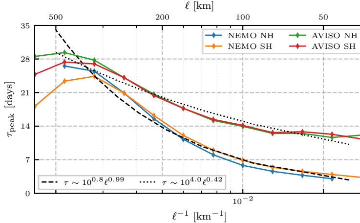
Figure 13. Mesoscale \tau - \ell Relationship For each filter scale ( \ell ), the time-scale ( \tau_{\text{peak}} ) for which the power spectrum ( -\partial_{\tau}\partial_{k_{\ell}}\mathcal{E}_{\ell,\tau} ) is maximized. While dashed lines show regression fits (see legend for regression formulas), which express \tau [s] in terms of \ell [m].
