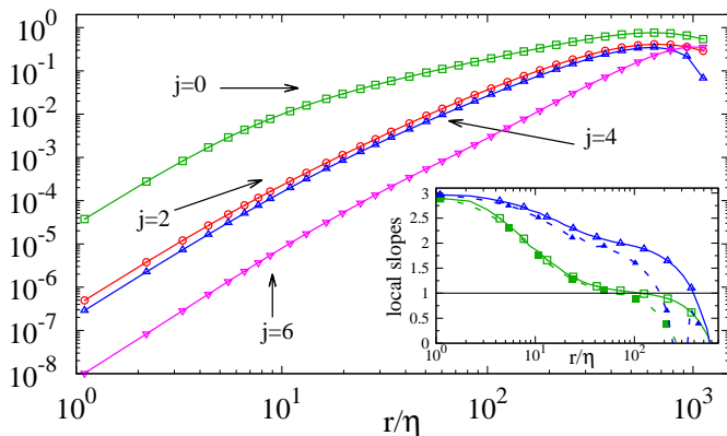
FIG. 2. Log-log plot of |S_{j,m}^{(3,L)}| vs r for different (j,m) sectors at R_\lambda = 450 . Symbols correspond to sectors (0,0) ( \square ), (2,0) ( \circ ), (4,4) ( \triangle ) and (6,6) ( \nabla ), respectively. Inset shows corresponding logarithmic local slopes for sectors (0,0) and (4,4) at R_\lambda = 300 (closed symbols) and R_\lambda = 450 (open symbols). Horizontal line at 1.0 is the exact result for sector (0,0) [41].
