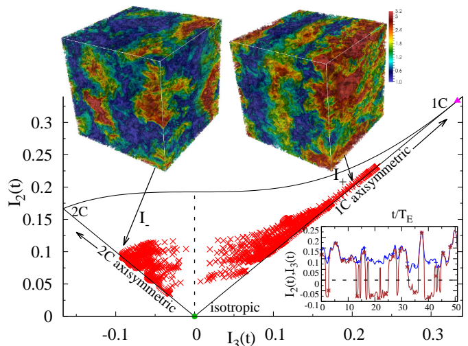
FIG. 1. Evolution of I_3, I_2 in the Lumley triangle ( \times ) for the 2048^3 RKF. The laminar state given by the forcing configuration is shown by ( \blacktriangle ). Inset shows steady-state evolution of I_2 ( + ) and I_3 ( * ) as functions of t/T_E . Reference line at zero is the isotropic state. Typical isocontours of the velocity magnitude in the 1C ( I_+ ) and 2C ( I_- ) regions are also shown.
